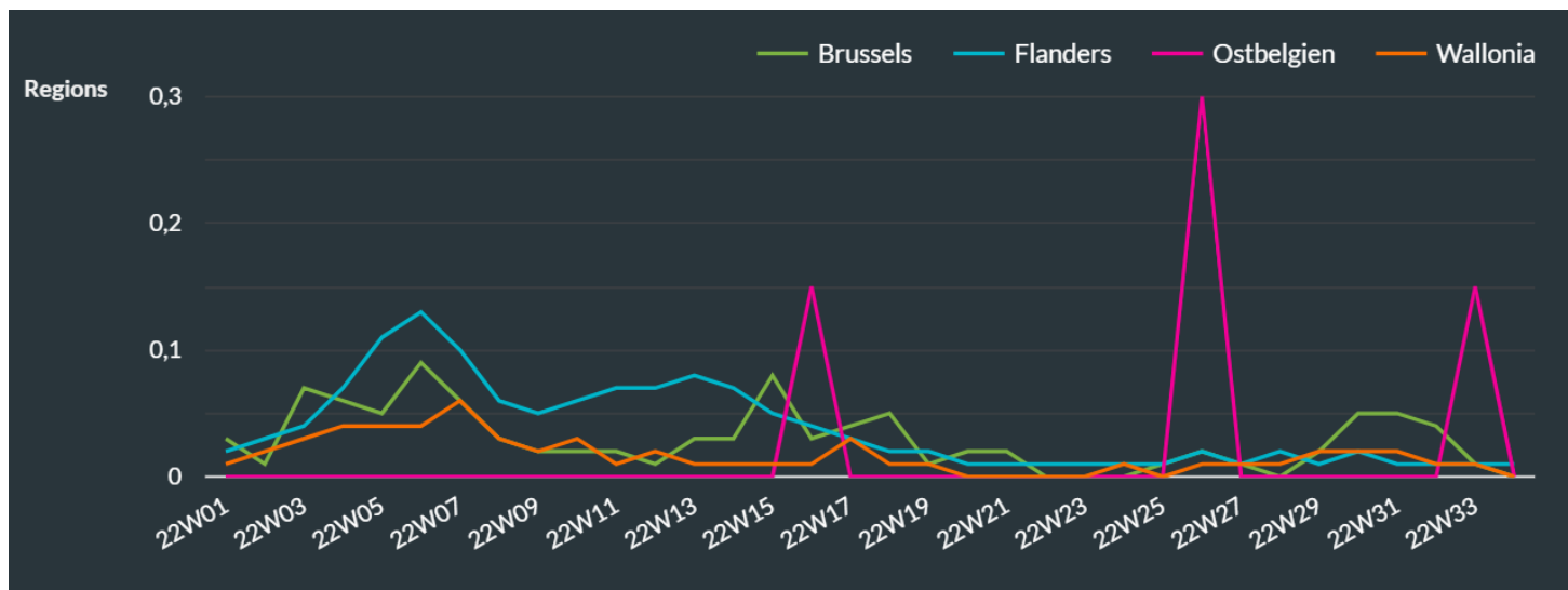
Deaths among possible, lab confirmed and radiologically confirmed cases per 100 residents (Dashboard Sciensano)
